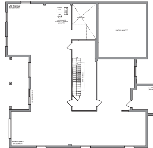
OPT. WALK-OUT BASEMENT - UNFINISHED (INCLUDES 308 SQ. FT. OF FINISHED BASEMENT) ELEVATION A
